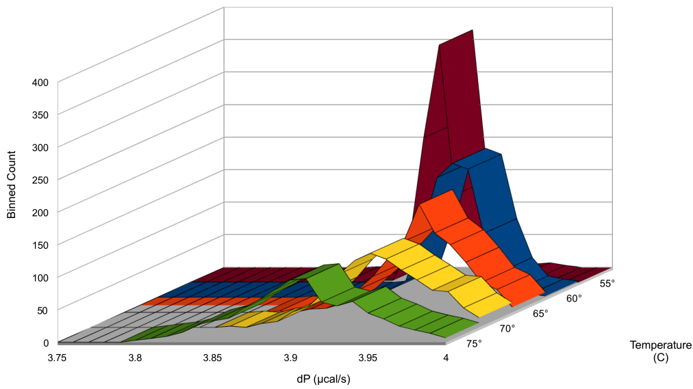
Baseline Noise Distribution iTC200 Water/Water, 43min.
