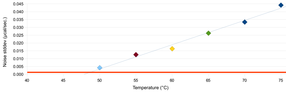
Baseline Noise iTC200 Water/Water
