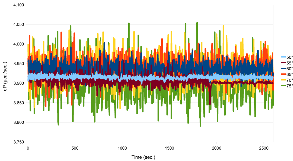
Baseline Noise iTC200 Water/Water
