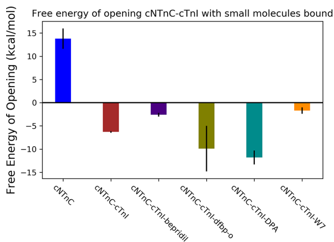
Figure 3. Umbrella sampling results of cNTnC–bepridil–cTnI, cNTnC–dfbp-o–cTnI, cNTnC–DPA–cTnI, and cNTnC–W7–cTnI systems. Free energies of opening were determined by WHAM analysis of umbrella sampling simulations. Small molecule-bound forms of cNTnC–cTnI-switch peptide complexes exhibited two responses to the presence of the small molecules. DPA and dfbp-o increased the relative stability of the open state of the complex more than cTnI by itself. Bepridil and W7 disrupted the relative stability of the open configuration of the cNTnC–cTnI complex. All values were calculated from triplicate simulations.
