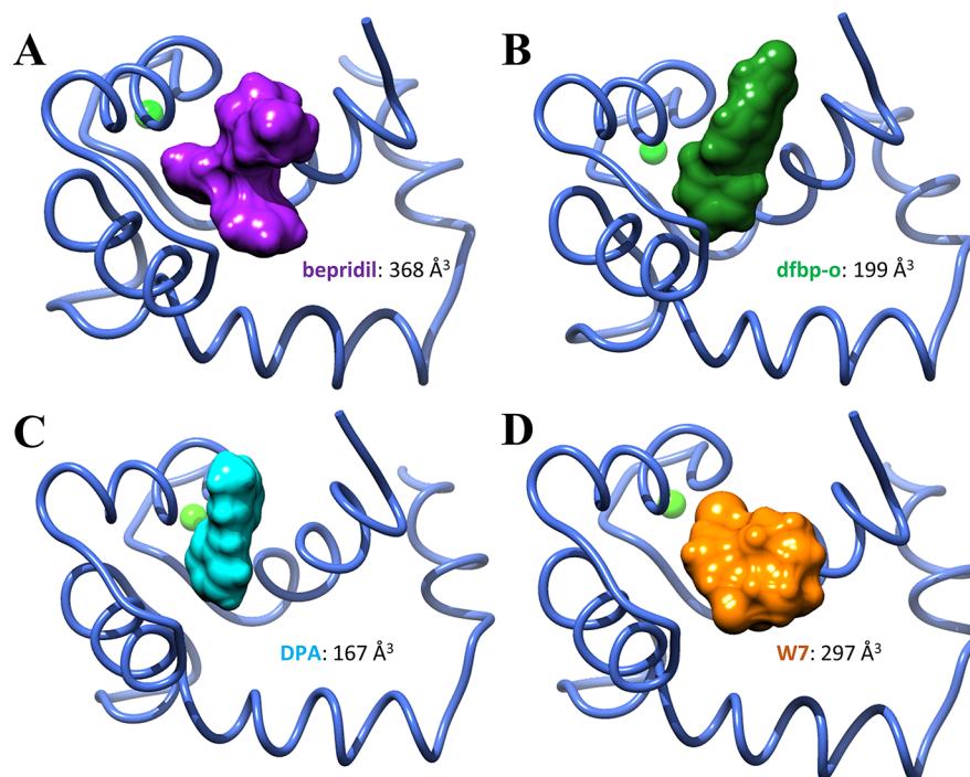
Figure 4. Volumes occupied by the small molecules bepridil, dfbp-o, DPA, and W7 bound to cNTnC. All of these small molecules lowered the relative free energy of opening when no cTnI was present in the simulations. Bepridil, with the largest occupied volume, lowered the relative free energy of opening to the greatest extent. The two small molecules that further increased the relative stability of the cNTnC–cTnI complex, dfbp-o and DPA, occupied the least amount of space, whereas bepridil and W7 occupied significantly more space and disrupted the relative stability of the cNTnC–cTnI complex.
