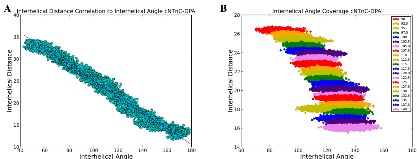
Figure 1. (A) Calculated interhelical angles plotted against interhelical distances from the frames of the steered MD of cNTnC–DPA. The two quantities were strongly correlated, suggesting that the interhelical distance can be used as an indirect measure of interhelical angle. (B) Interhelical angles and distances were calculated for each of the windows in the umbrella sampling simulations of cNTnC–DPA and plotted against each other. There was sufficient overlap between the angles to ensure adequate sampling.
