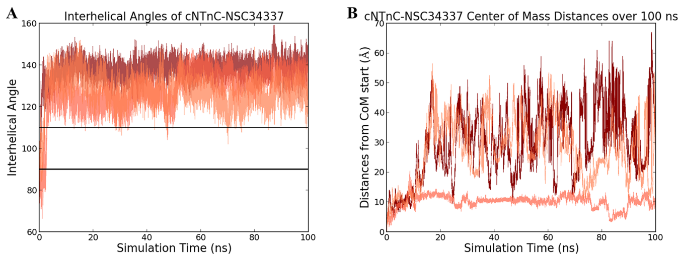
Figure 5. (A) Interhelical angle calculated for triplicate 100 ns molecular dynamics simulations of predicted poor binder NSC34337 bound to cNTnC. In all three simulations, the small molecule left within less than 3 ns of the simulations, allowing cNTnC to close immediately. (B) Center-of-mass distances for cNTnC–NSC34337 over triplicate 100 ns molecular dynamics simulations from the starting position. NSC34337 left the hydrophobic pocket immediately, resulting in a loss of all key binding interactions seen for the known binders.
