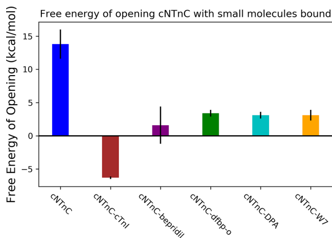
Figure 2. Umbrella sampling results of cNTnC–bepridil, cNTnC– dfbp-o , cNTnC–DPA, and cNTnC–W7 systems. Free energies of opening were determined by WHAM analysis of umbrella sampling simulations. Small molecule-bound forms of cNTnC exhibited a lower relative free energy of opening compared to the corresponding small molecule-free system. These values were calculated from triplicate simulations.
