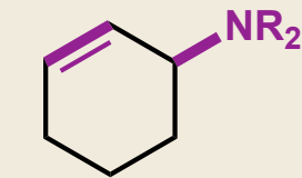
intermolecular desaturative amination triple C-H
