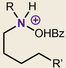
unprotected amines
