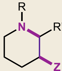
\delta desaturation to heterocycles double C-H
