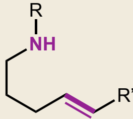
\delta desaturation to heterocycles double C-H
