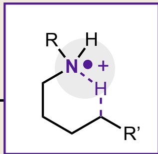
polarity matched HAT via N-radical cations
