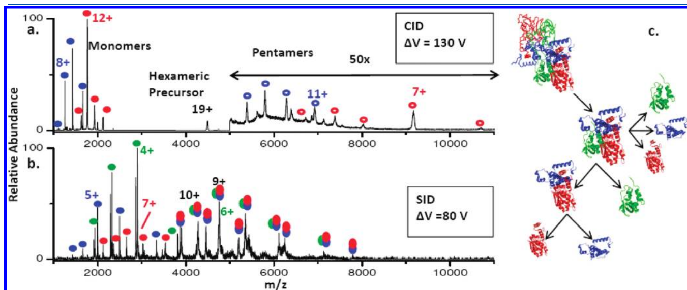
Figure 2. Comparison of (a) CID and (b) SID spectra for TNH. In the SID pathway schematic (c), each subunit in the structure (the homologous thiocyanate hydrolase) is indicated by a different color for clarity: \alpha , red; \beta , blue; and \gamma , green. In (a) and (b), monomeric product ions are indicated by a solid circle of the corresponding color, while the complementary pentamers are indicated by an open circle of the same color as the monomer. In (b), the data from the homologue shown in (c) has been applied to the labeling scheme, as such, subcomplexes are indicated by clusters of the appropriate color circles.
