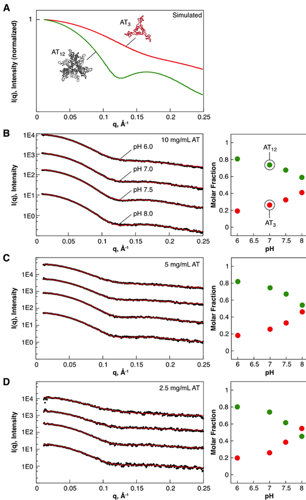
Fig. 5. SAXS profiles of AT can be described as mixtures of AT 3 and AT 12 . A, scattering curves for AT 3 and AT 12 , computed from the dodecameric crystal structure (2bx9). B-D, left, experimental scattering intensities (black) for AT recorded over a range of pHs (6, 7, 7.5, 8) and concentrations (1.77, 0.89 and 0.44 mM), fit to a two-state model with varying fractions of AT 3 and AT 12 . Profiles are offset in the y-axis from each other for visibility. Right, fitted volume fractions as a function of pH for each sampled concentration.
