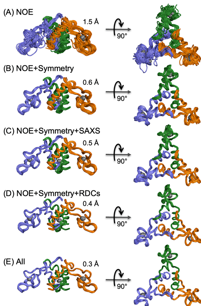
Fig. 8. Impact of restraint classes on precision of AT 3 NMR ensemble. Each ensemble was computed using NMR-derived torsion angle restraints, and (A) NOEs, (B) NOEs and three-fold symmetry restraints, (C) NOEs, symmetry, special restraints from SAXS data, (D) NOEs, symmetry restraints and residual dipolar couplings, and (E) all restraint classes. Backbone RMSDs as indicated.
