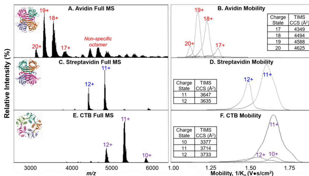
Figure 3. Full mass spectra and extracted mobility distributions with experimental CCS values (single measurements) for 20 \mu\text{M} avidin (A, B, PDB 1AVE) in 200 mM ammonium acetate, 5 \mu\text{M} streptavidin (C, D, PDB 1SWB) in 160 mM ammonium acetate and 40 mM TEAA, and 5 \mu\text{M} CTB (E, F, PDB 1FGB) in 160 mM ammonium acetate and 40 mM TEAA.
