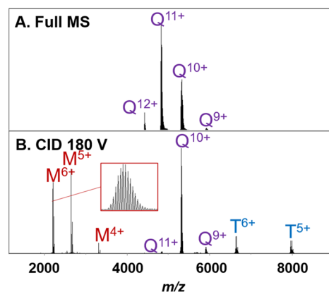
Figure 4. Streptavidin tetramer (5 \mu\text{M} ) in 160 mM ammonium acetate with 40 mM TEAA full MS (A). Collision cell CID 180 V of the entire tetramer charge state distribution (B). Initial precursor ions in panel (A) are labeled Q for tetramer with their corresponding charge state. In panel (B), remaining tetramers are also labeled Q, with fragment ions labeled M for monomeric ions or T for trimeric ions with corresponding charge states.
