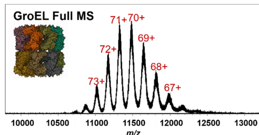
Figure 6. Full MS of GroEL ( 5 \mu\text{M} ) in 200 mM ammonium acetate.
