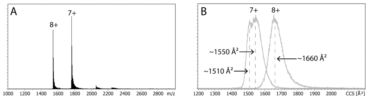
Figure 2. Full ESI mass spectrum (A) and extracted mobility distributions (B) for 30 \mu M cytochrome c in 10 mM aqueous ammonium acetate solution.
