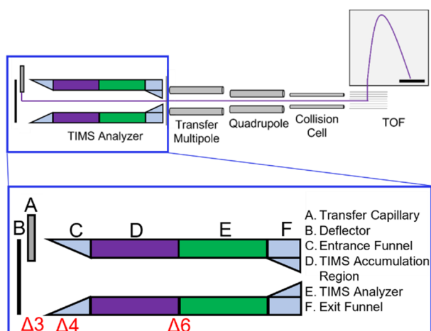
Figure 1. Overview of the timsTOF Pro instrument. Mobility analysis is performed in the TIMS analyzer, followed by a transfer multipole, quadrupole (selection up to 3000 m/z ), collision cell, and time-of-flight (TOF) mass analyzer. The purple trace indicates the path of ion motion. Delta values represent potentials set in the source/TIMS region, with \Delta 3 being the voltage difference between the Deflector and Entrance Funnel, \Delta 4 being the voltage across the entrance funnel, and \Delta 6 being the voltage applied between the exit of the TIMS accumulation region (purple) and the entrance of the TIMS analyzer region (green). Optimization of these potentials for high molecular weight operation is discussed in the main text.
