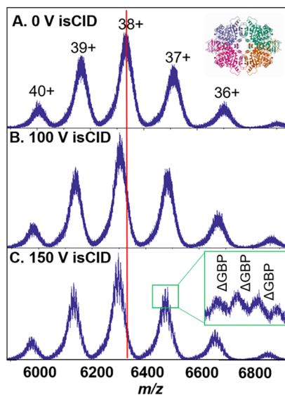
Figure 5. Full mass spectra of pyruvate kinase ( 5 \mu\text{M} ) in 200 mM ammonium acetate with increasing amounts of in-source activation (isCID) to remove nonspecific adducts. As adducts were lost, the m/z apex of each charge state decreased as demonstrated by the red line placed at the apex of 38+ for no activation (A–C). At high isCID, GBP adductions began to be resolved.
